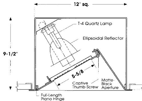
CROSS SECTION (9930 Illustrated)
