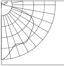
BIS1001XX-ELE-GEP TEST NUMBER: 26246 LAMP: 100W A19 LUMENS: 1,680 MOUNTING HEIGHT: 12 FEET
