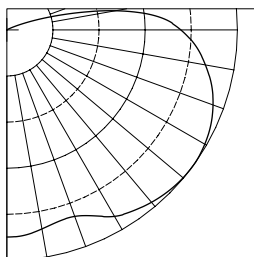
BIS175MXX-SUZ-GEP TEST NUMBER: 26253 LAMP: 175W MH, COATED LUMENS: 15,000 MOUNTING HEIGHT: 12 FEET
