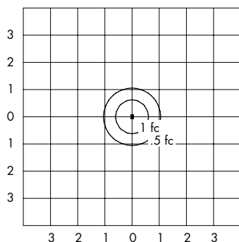
BIS100IXX-SUZ-GEP TEST NUMBER: 26252 LAMP: 100W A19 LUMENS: 1,680 MOUNTING HEIGHT: 12 FEET
