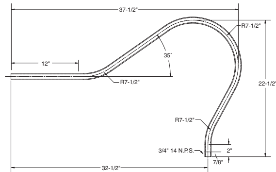
W3D = 3/4" Stem Style
