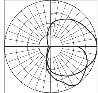
KALEIDOSHADE 2 MEDIUM DEEP ANGLE REFLECTOR, LAMP @ 1 POSITION VENTURE MA175/C/U COATED IES Test # K2E175MCG
