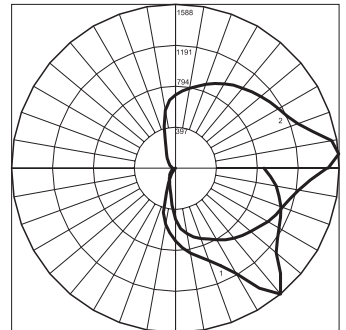
KALEIDOSHADE 2 MEDIUM DEEP ANGLE, LAMP @ 1 POSITION PHILIPS 200 WATT INC FROSTED IES Test # K2E200IG
