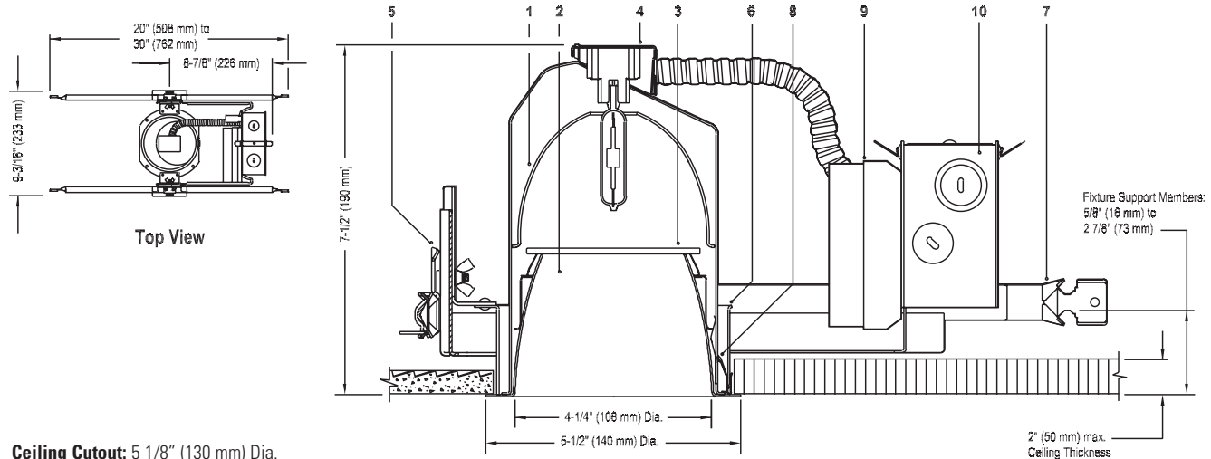
Ceiling Cutout: 5 1/8" (130 mm) Dia.
