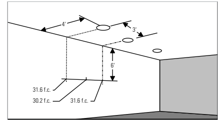
Lighting Data - Example C6E17OWCLW illumination on the wall 6' down from the ceiling is 31.6 f.c. beneath and 30.2 f.c. between fixtures.
