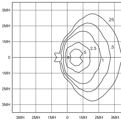
FPS150NLXL-1 @ 45°
