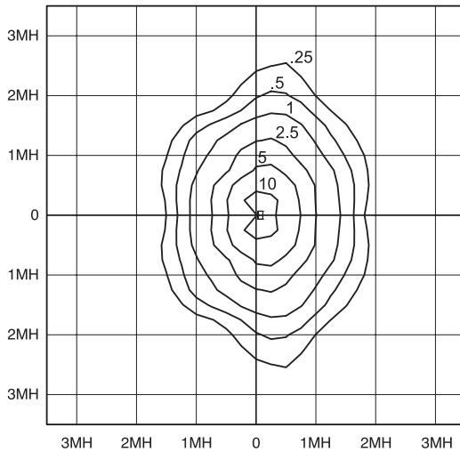
FPS150NLXL-1 @ 0°
