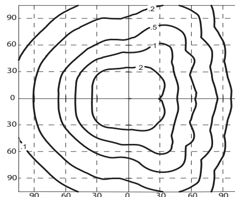
SSH3400LX
