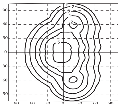
SSH2400PMA
