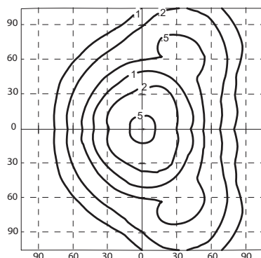
SSH3400PMA
