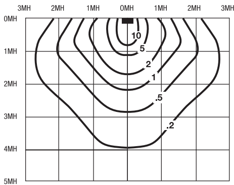
WP250MA (Quick Ship Number WP251MA) MH250/U 20,500 Lumens 15' Mounting Hgt.
