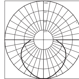
KALEIDOSHADE 2 LARGE SHALLOW FLUTED REFLECTOR, PHILIPS 300 WATT INC COATED PS-35 LAMP IES Test # K3F300IG
